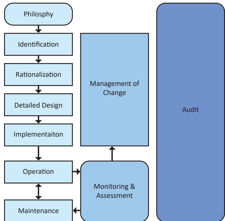
Alarm rationalization work process
