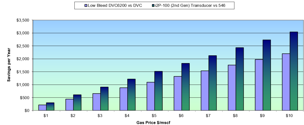
Annual Natural Gas Savings with Fisher Low Bleed DVC6200 and i2P-100 (2nd Gen)
